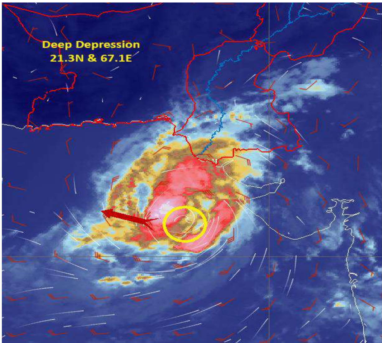
Satellite image (2 nd October 2025, 1030 PST)
